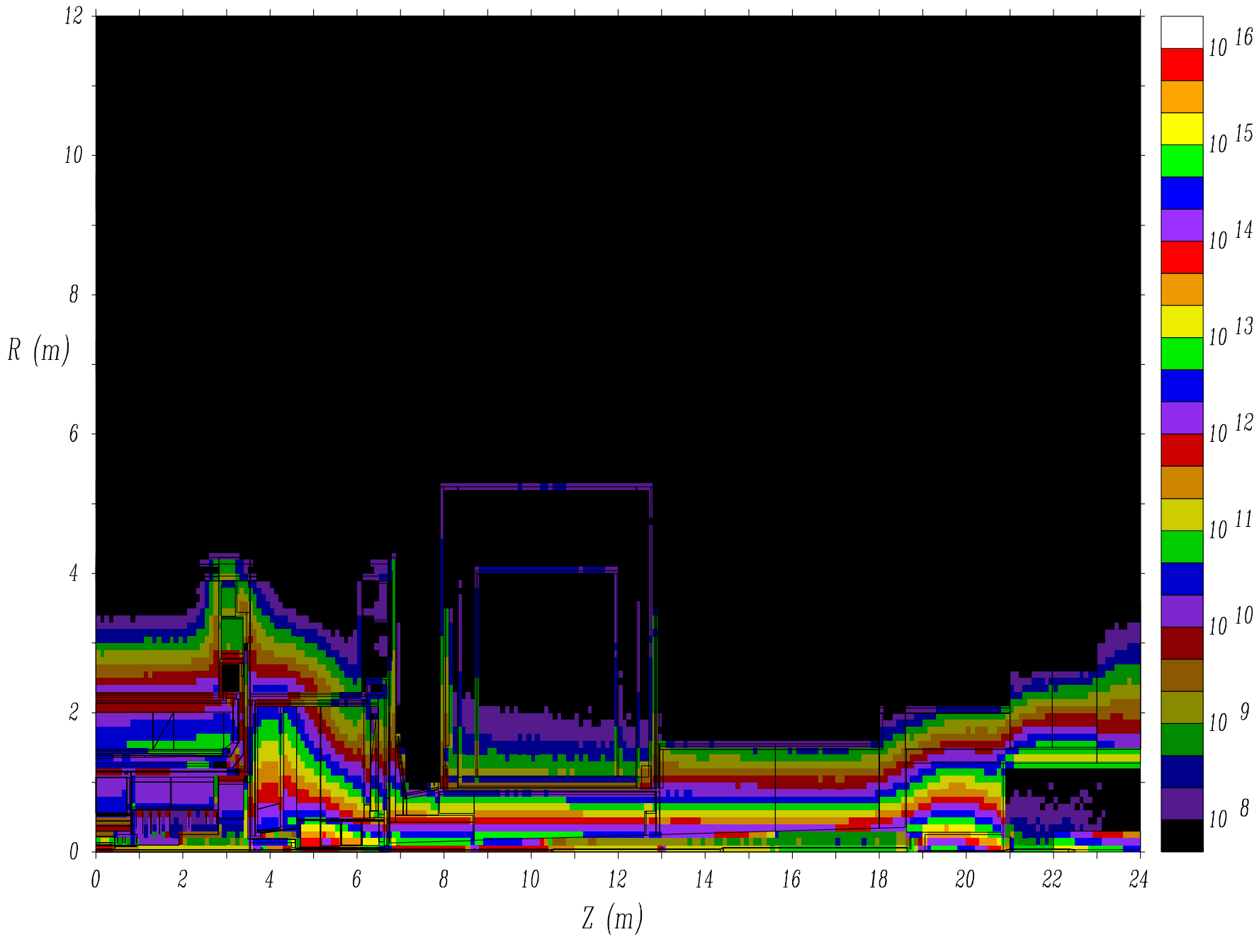
Jan03 Base (24620) - Star Density, N/cm^3/Yr
