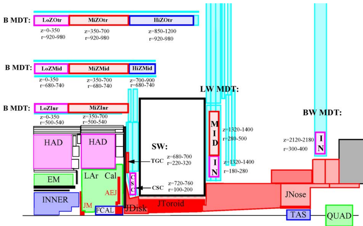
Figure 8.2 The scoring regions in the muon spectrometer used in the optimization studies.
