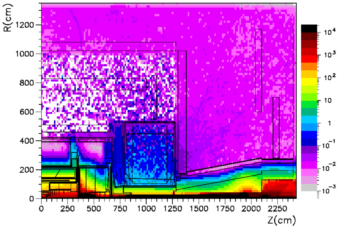
Figure 6.31 Electron fluences with and without muon chamber material
