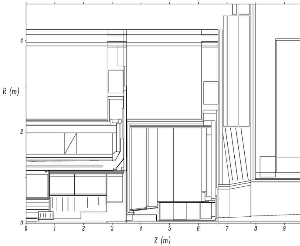
Figure 4.13 GCALOR TP43 geometry: calorimeter region.
