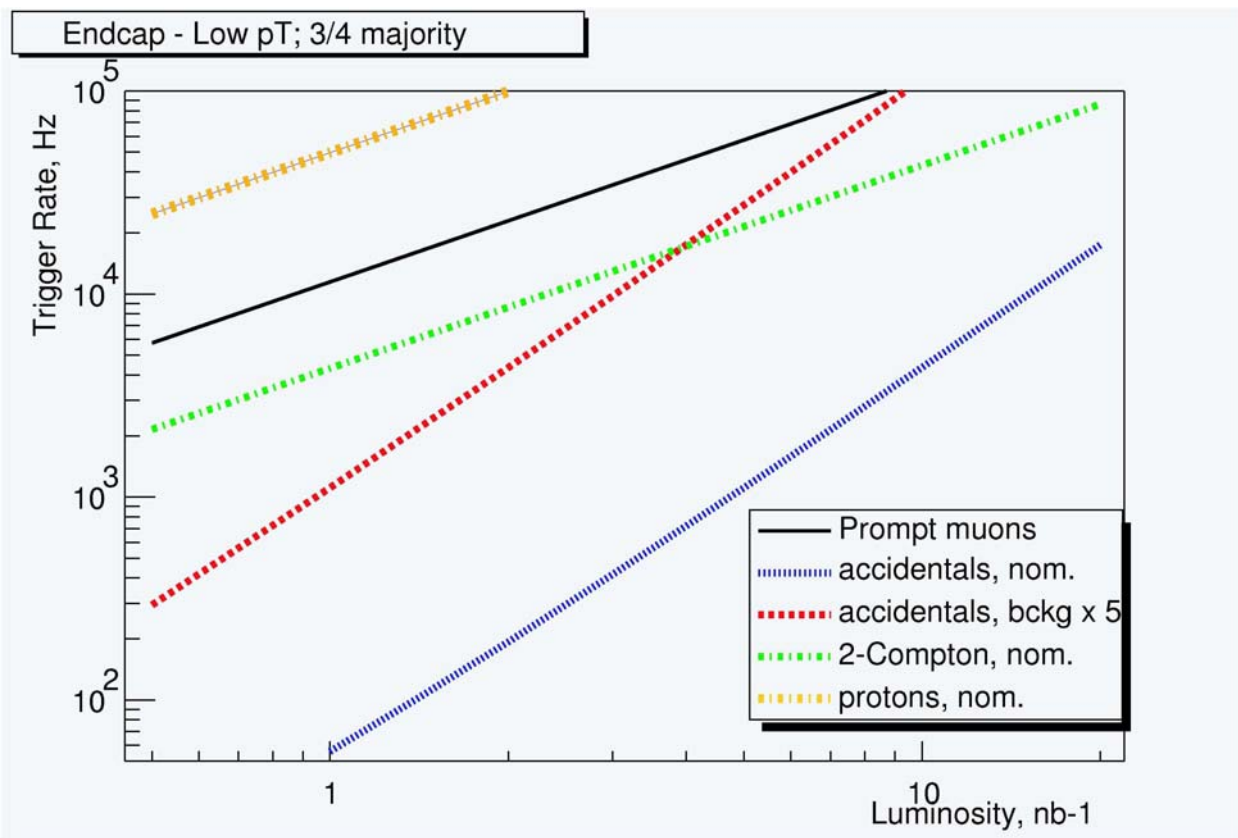
Figure 6.35 Low pT Trigger rates estimates done with the fluxes predicted by Gcalor and with the efficiencies obtained for the Gcalor energy spectra. In the case of charged particles, currents are used instead of fluxes using the flux-to-current conversion factor from Table 5.11.
