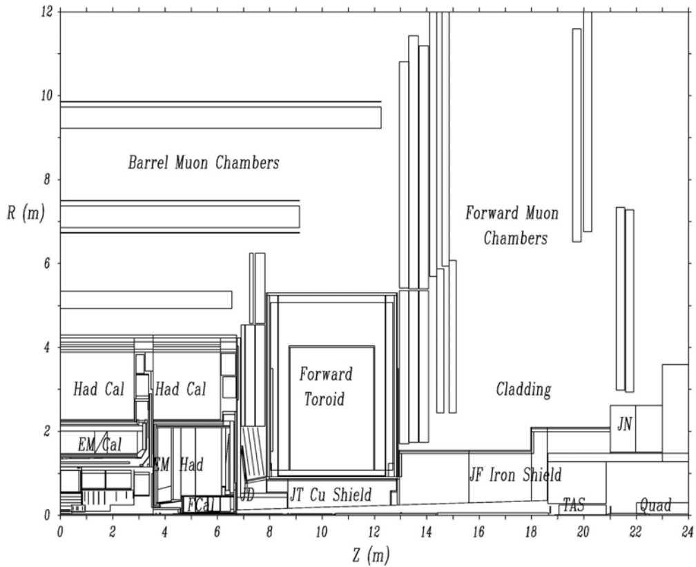
Figure 4.16 A full quadrant of the Atlas “Jan03” geometry layout as modeled with GCALOR. The picture shows all structures in phi projected into one plane. The old muon chambers positions have been kept for backward compatibility with earlier versions.
