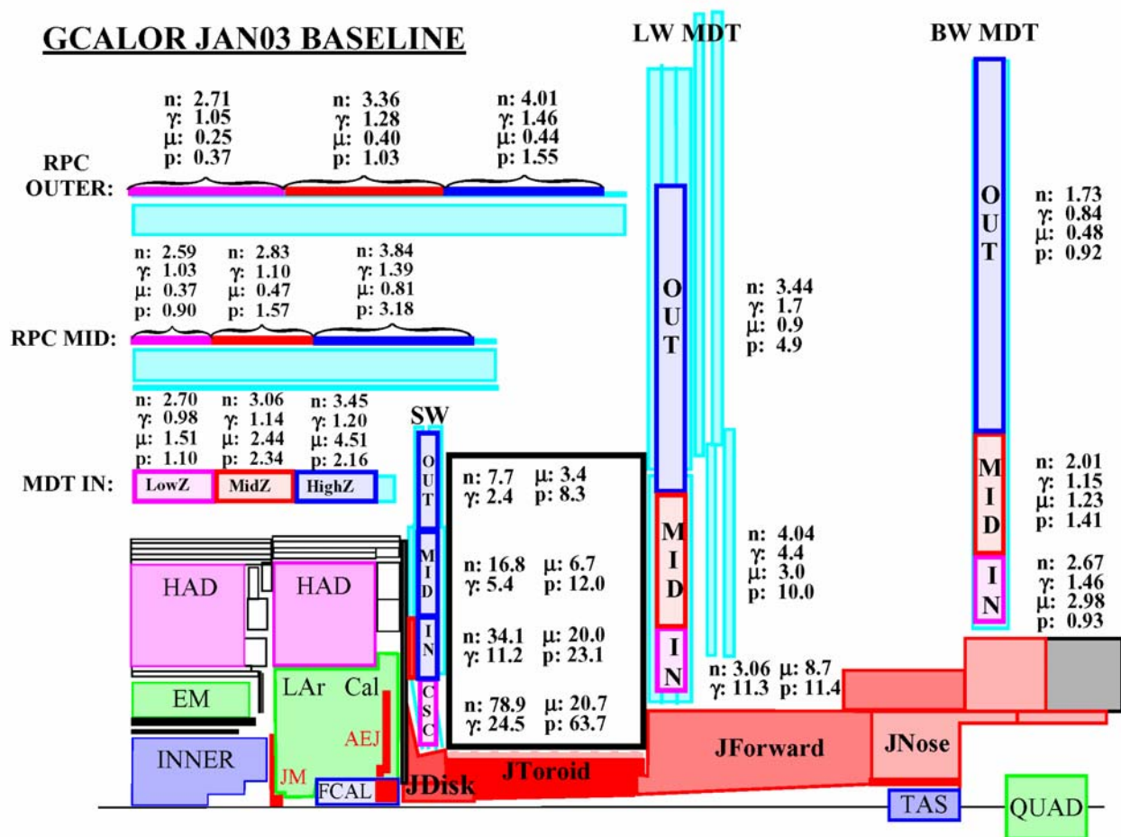
Fig. 3 Fluences in the muon chamber locations at high luminosity ( 10^{34} \text{ cm}^{-2} \text{ s}^{-1} ) as predicted by GCALOR for the Jan03 layout. The n and \gamma fluences are in units of \text{kHz/cm}^2 and the \mu and p fluences in \text{Hz/cm}^2 .
