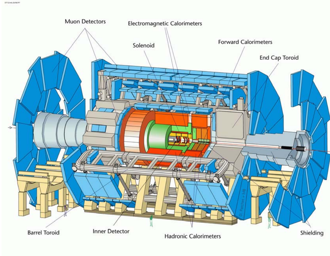
Figure 1.1 Overall layout of the ATLAS detector
