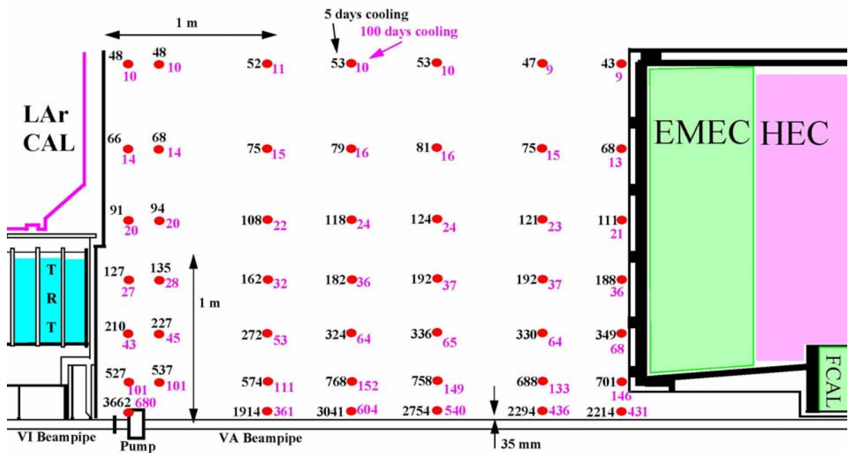
Figure 9.7 The doserate between the inner detector and the endcap calorimeter during the standard access scenario. Values are given for both 5 and 100 days of cooling-off. Calculation by Morev et al. [122].
