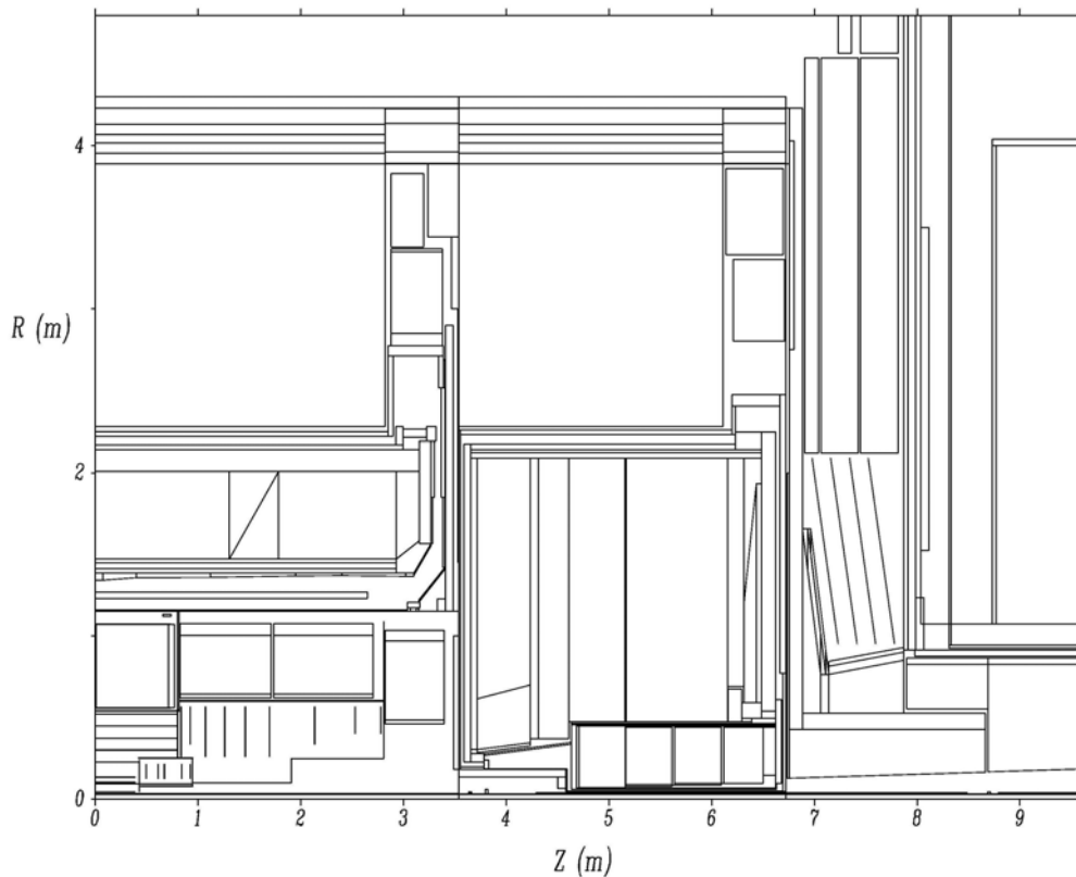
Figure 4.17 Zoomed view to the calorimeter region in GCALOR “Jan03” layout.
