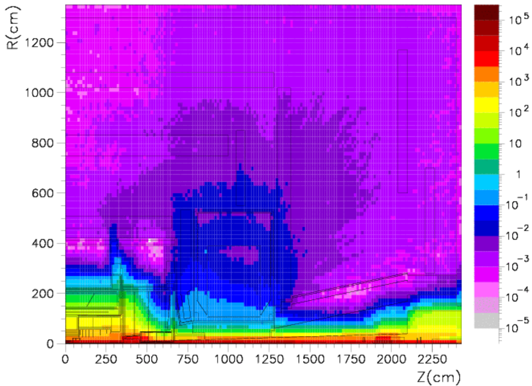
Figure 6.15 Charged hadrons (dominated by protons) as predicted by FLUKA
