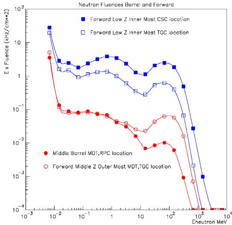
Figure 6.11 Neutron fluences in various regions of the muon spectrometer: all neutrons with energies below 10 keV are collapsed in a single bin. There are 6 orders of magnitude (or 12 bins) down to the thermal neutron energy.
