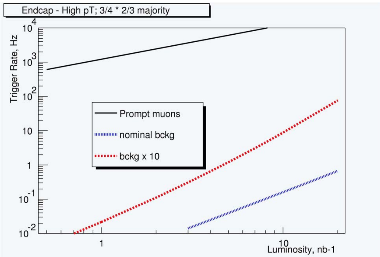
Figure 6.36 High pT Trigger rates estimates done with the fluxes predicted by Gcalor and with the efficiencies obtained for the Gcalor energy spectra. In the case of charged particles, currents are used instead of fluxes using the flux-to-current conversion factor from Table 5.11.
