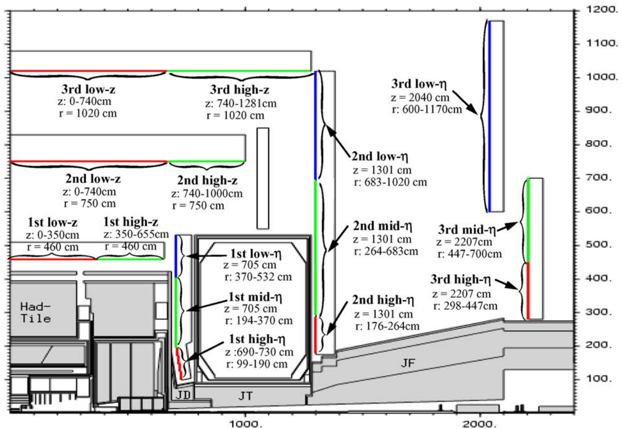
Figure 5.16 Scoring surfaces used by FLUKA to quote background rates in Table 5.10.
