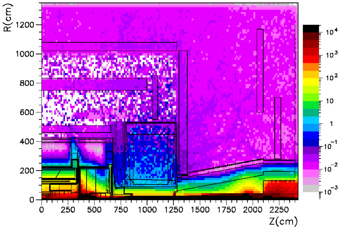
e^+ fluences ( \text{kHz}/\text{cm}^2 ) for av16 geometry
