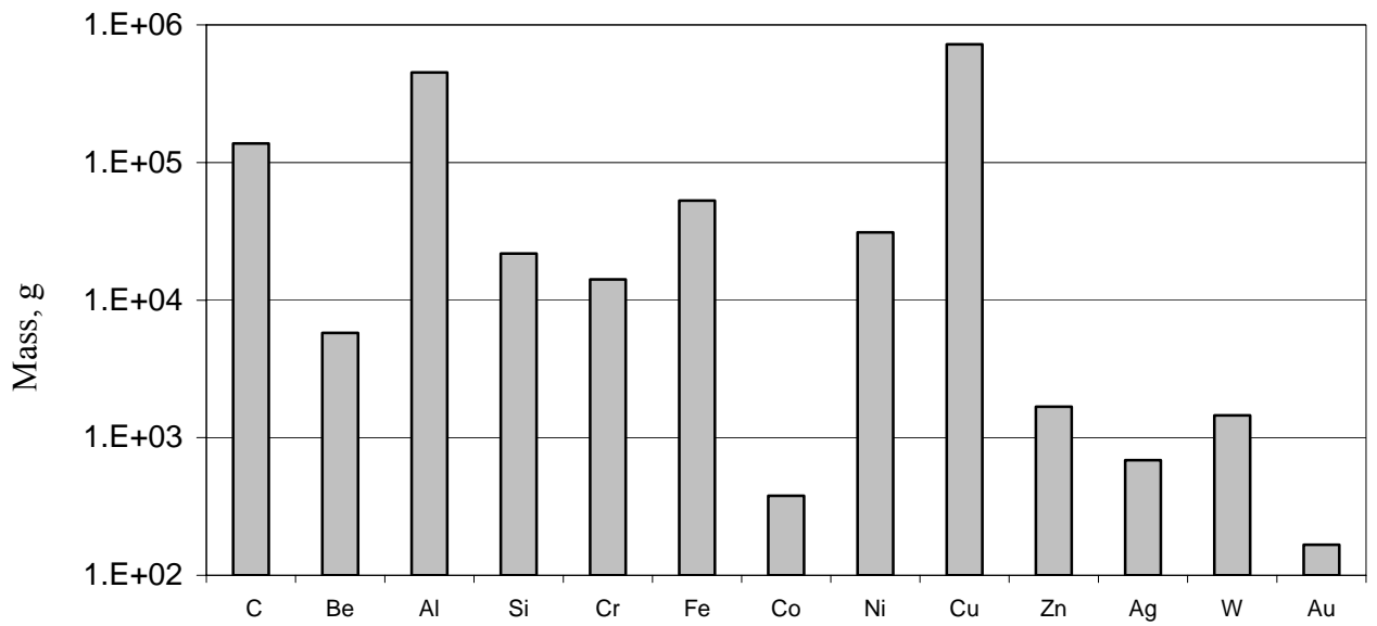
Fig. 4 Material break down of Inner Detector
