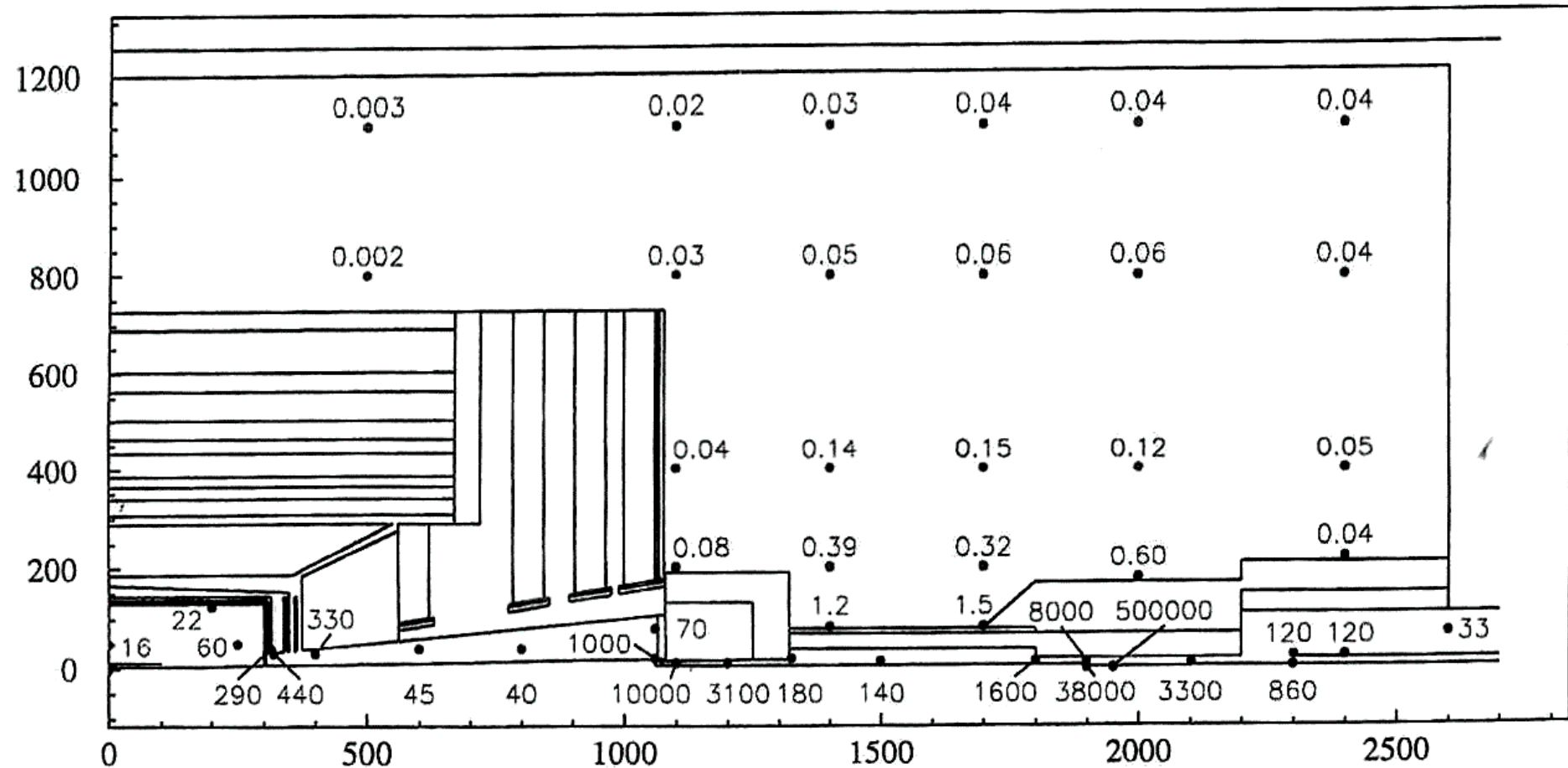
Estimated dose rates from induced radioactivity (in \mu\text{Sv/h} ) 1 day after the stop of a 60 day operating period
