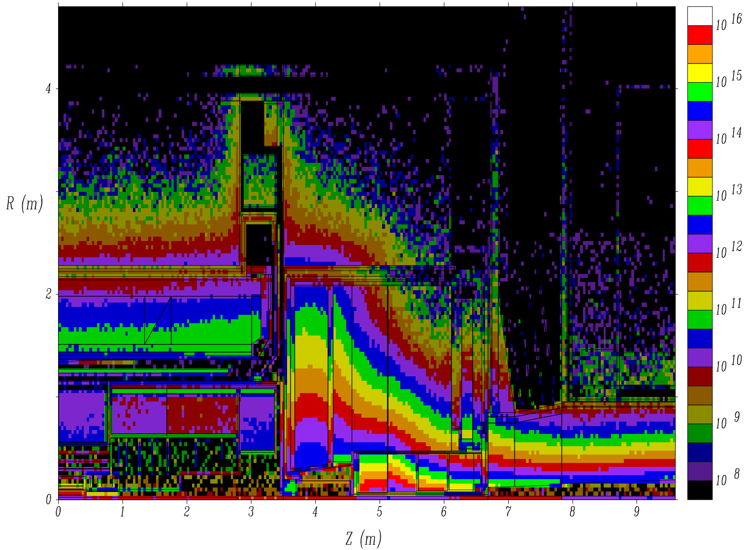
GCALOR TP43 Comparison (1624) - Star Density, N/cm^{**3}/Yr
