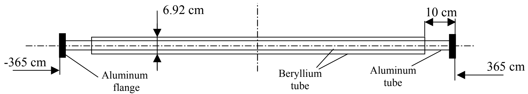
Fig. 1 Sketch of the ID Beam pipe section.
