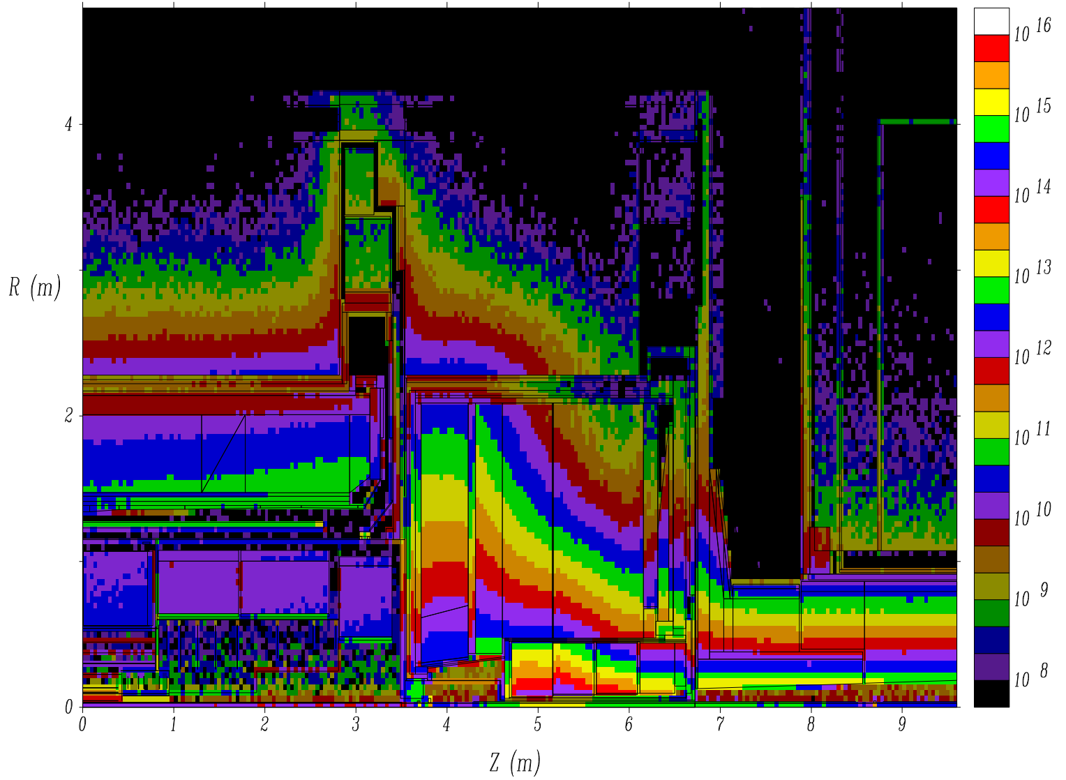
ATLAS Aug01 Baseline (5992) - Star Density, N/cm^3/Yr
