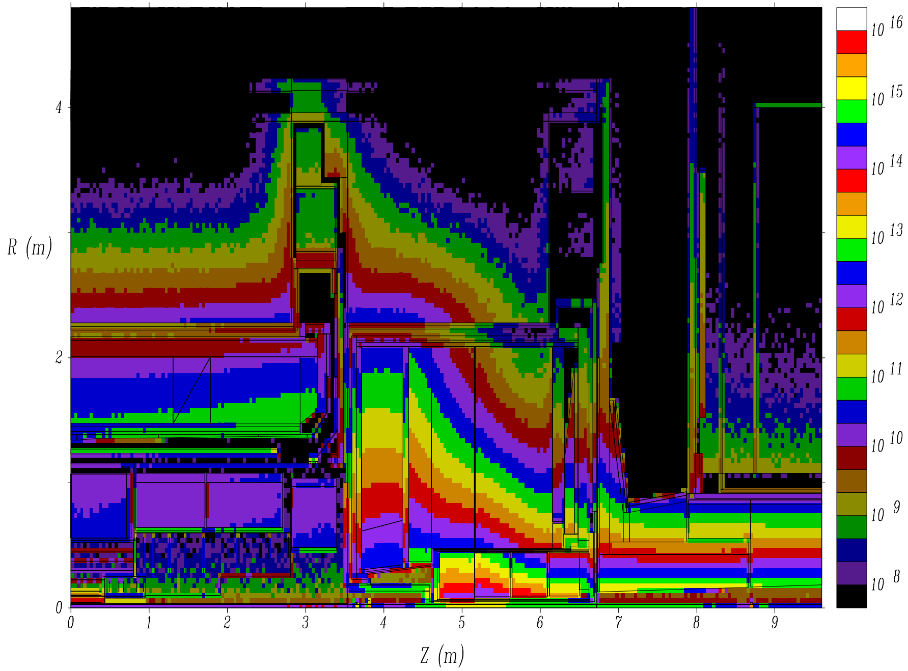
Jan03 Base (24620) - Star Density, N/cm^3/Yr
