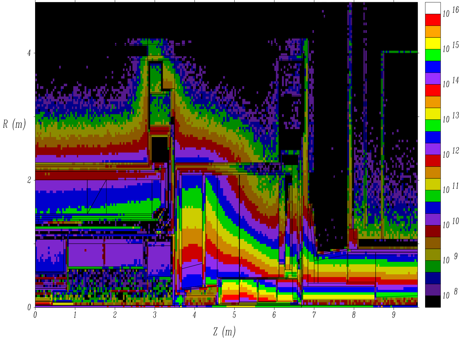
June JDCu JT4cm (6004) - Star Density, N/cm**3/Yr
